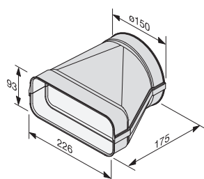
Adapter DFK-A
